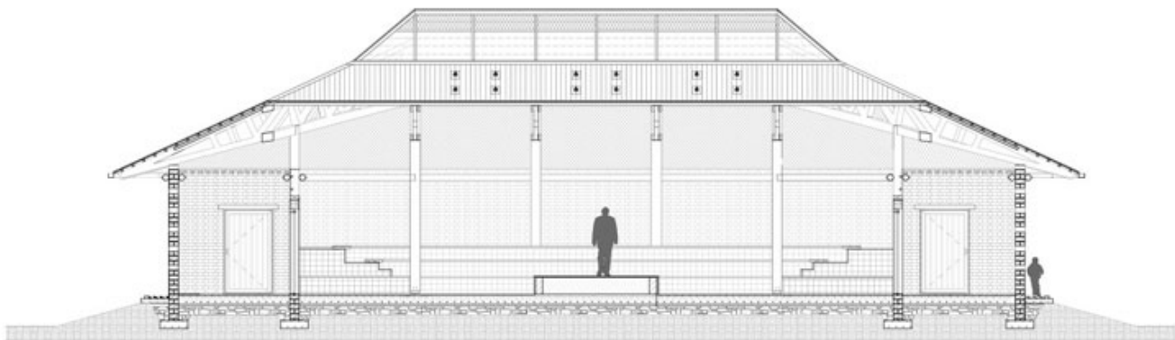
Sections
