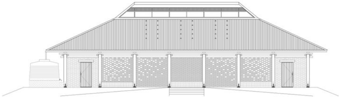
Elevations
