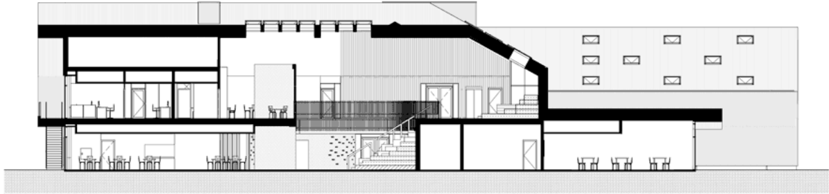
SECTION NORTH-SOUTH - EDUCATIONAL SPACES
