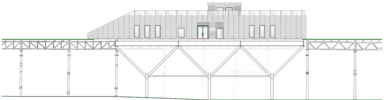
VISITOR CENTRE- WEST ELEVATION
