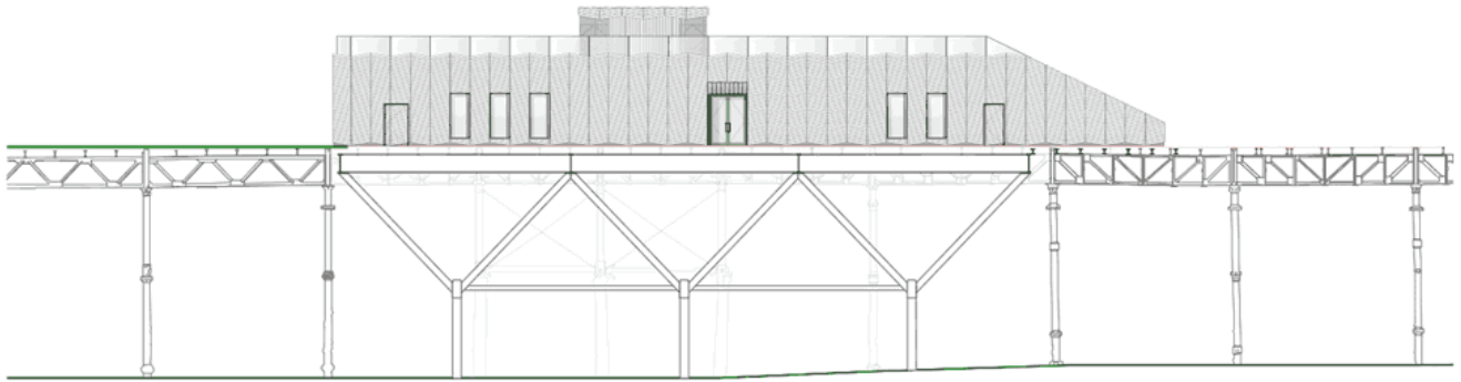
VISITOR CENTRE- EAST ELEVATION
