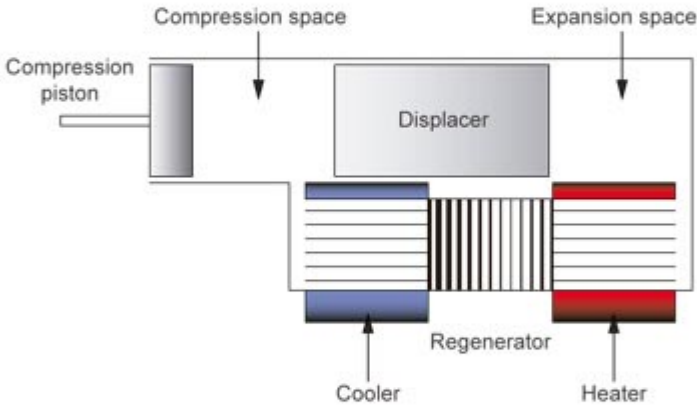
Gamma engine
