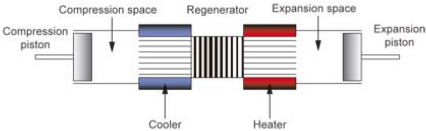
Beta engine
