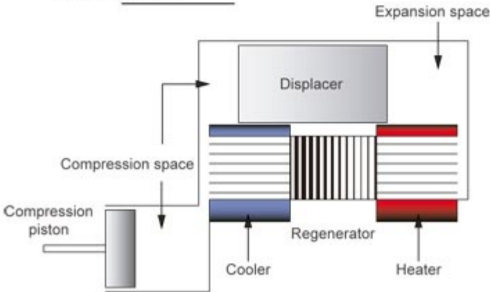
Gamma engine
