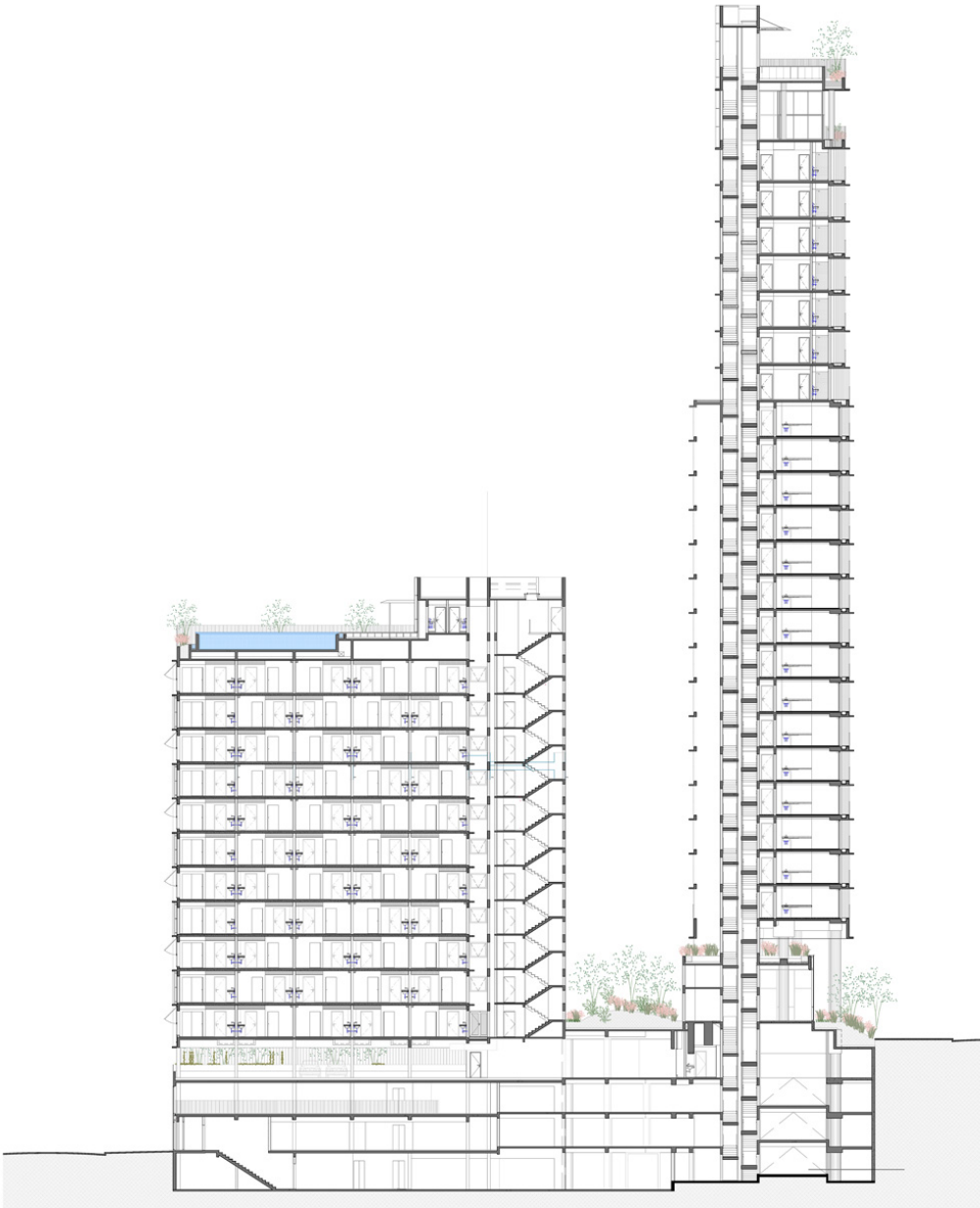
AA SECTION 1:100 0 5 10 20 30m
