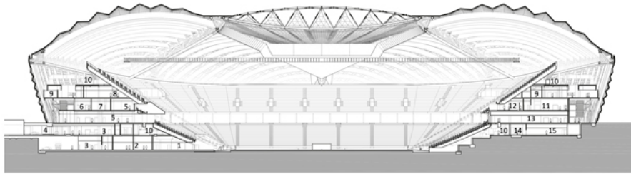
East-West Section - Tournament Mode Capacity: 40,000
